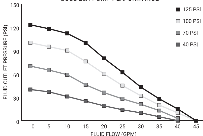
GOSS 25A PUMP PERFORMANCE
